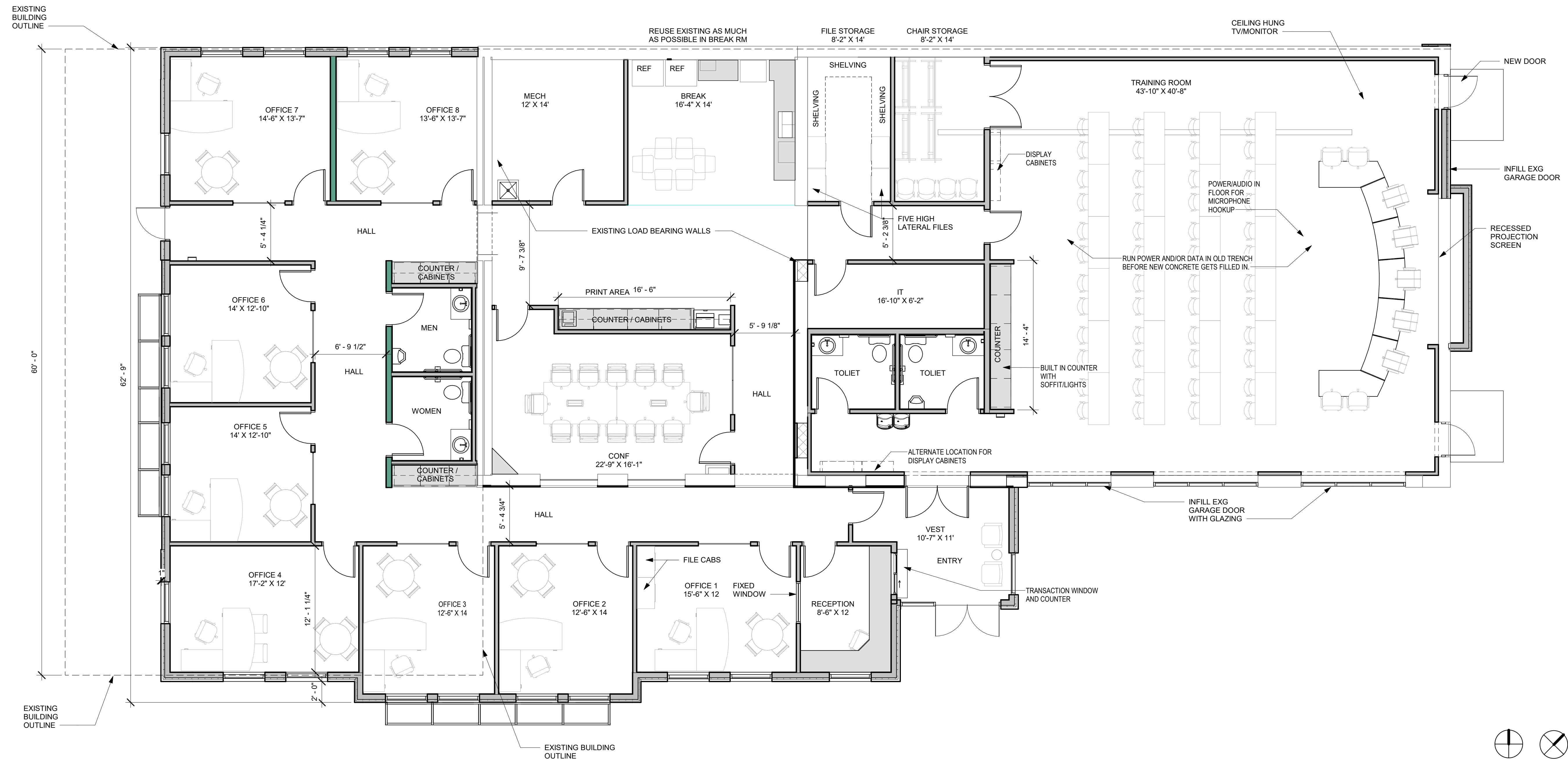
1 Floor Plan - Presentation 3/16" = 1'-0"
